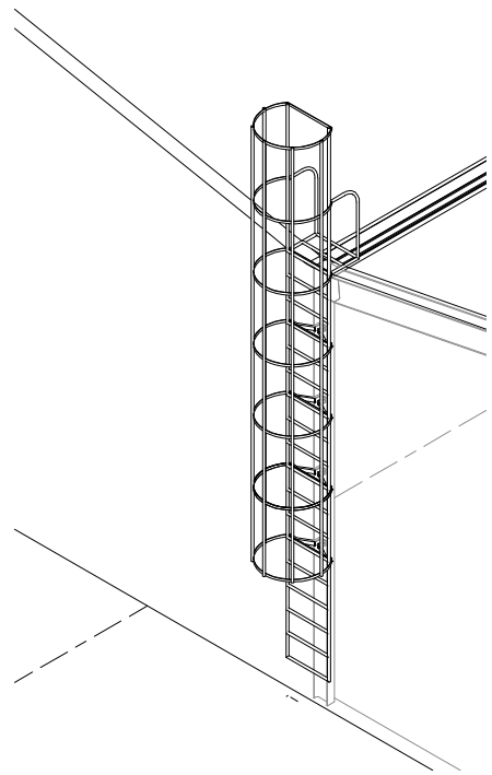
5 ISOMETRICA AP01
